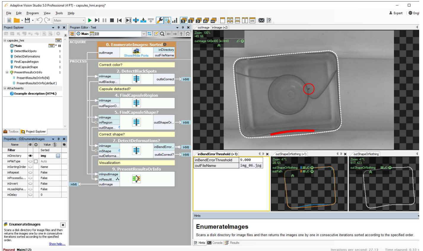
The Main Window of Adaptive Vision Studio.
